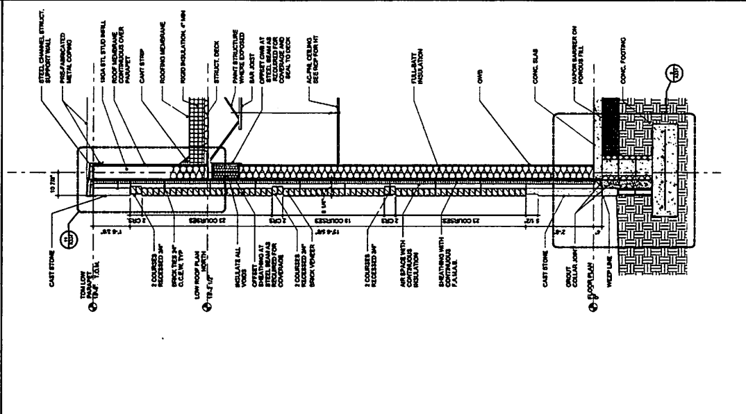
1 TYPICAL METAL STUD WALL SECTION SCALE: 3/4\"/>
