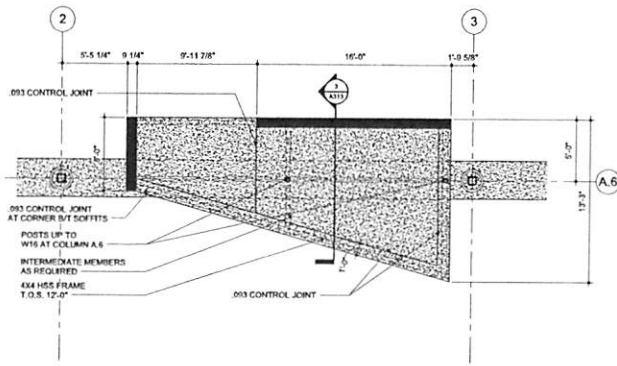
2 SOFFIT ABOVE RECEPTION DESK SCALE: 1/4" = 1'-0"
