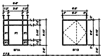
8 FRAME ELEVATIONS- SF1A SCALE: 1/4" = 1'-0"
