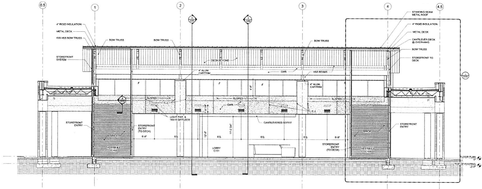
1 BUILDING SECTION 3 SCALE: 1/4" = 1'-0"
