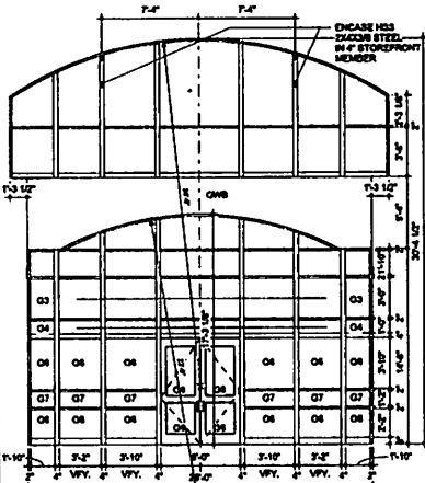
5 FRAME ELEVATION- SF2A SCALE: 1/4" = 1'-0"
