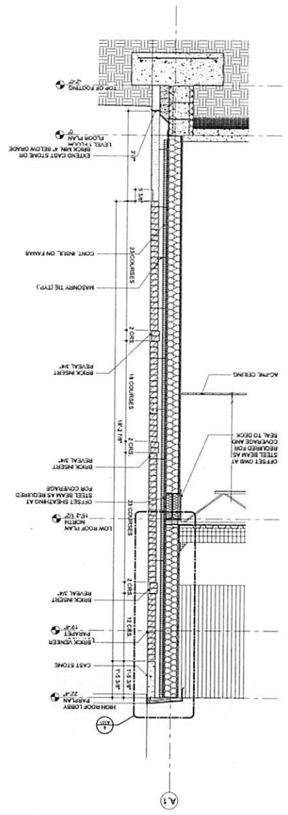
1 HIGH WALL SECTION SCALE: 3/4" = 1'-0"
