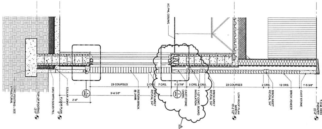
2 TYPICAL SHELTER WINDOW SECTION
