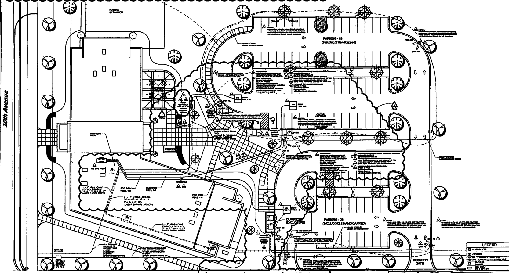
EDGE BUILDING SECURITY CAMERA SITE LAYOUT DRAWING
